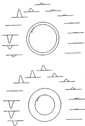
Fig. 2. Coronal scalp distribution of a tangential dipole modeling fusaral cortical activity. As explained for figure 4, the correctly transformed eccentricity in the homogeneous head model (bottom) results in a realistic scalp topography with widespread positive and negative maxima to either side of the actual location of the source. Note that in the quasistatic approach a single dipole source contributes the same waveform at all electrodes. Only the sinusoidal factor and the sign vary with electrode site.
