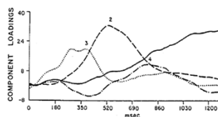
Figure 10-4. Plot of four sets of component loadings derived from a principal-components analysis (PCA) of an ERP data set. Each of the component loading vectors is composed of 128 points corresponding to 128 time points (100-Hz digitizing rate) in the waveforms.
