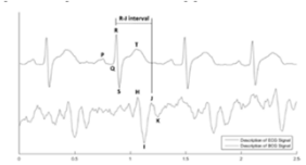
Figure 1. Location of P, Q, R, S, and T peaks in ECG and H, I, J, and K peak in BCG signal. The x-axis represents time (sec), and the y-axis is expressed in arbitrary units.
