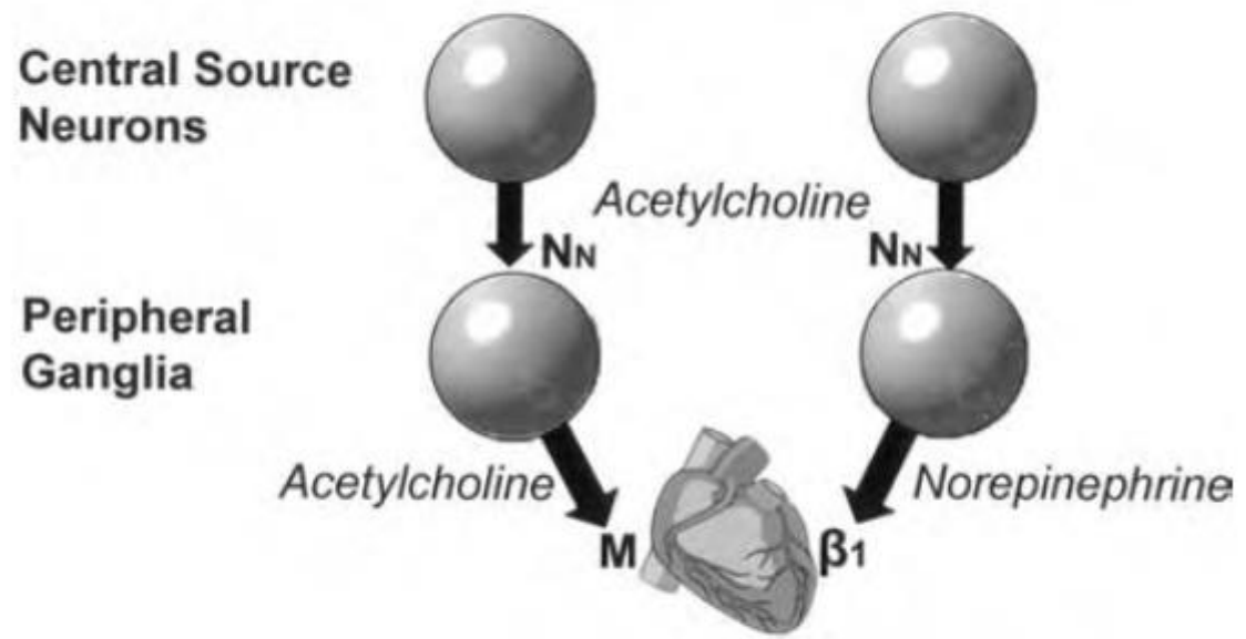
Figure 8.6. General pattern of pharmacology of the autonomic innervations. Abbreviations refer to the relevant postsynaptic receptor populations: N_N – nicotinic cholinergic; M – muscarinic cholinergic; \beta_1 – beta1 adrenergic.
